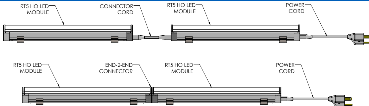
Standard Mount (MT5-MC-000)
